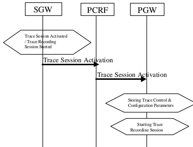
Figure 4.1.2.10.1.A illustrates the Trace Session activation in case of PMIP based S5 interface. The figure contains only the difference compare to the GTP based S5 interface
