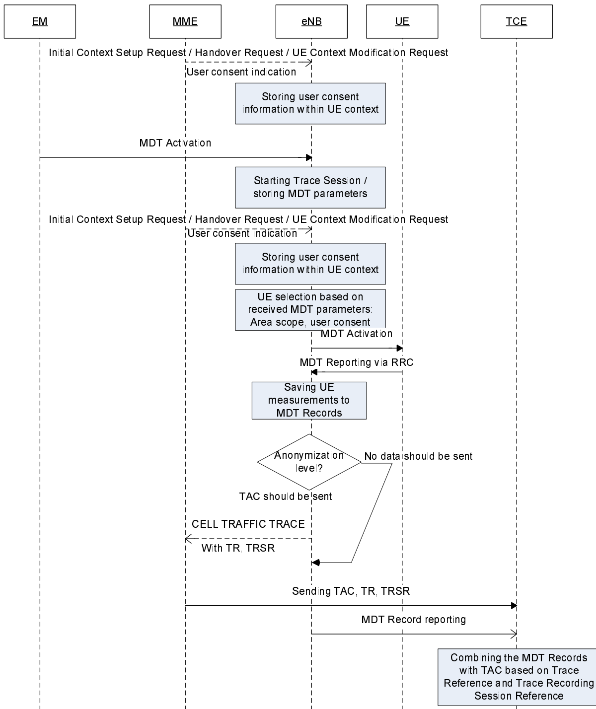
Figure 4.1.1.6a.1 Example for area based logged MDT activation in E-UTRAN
