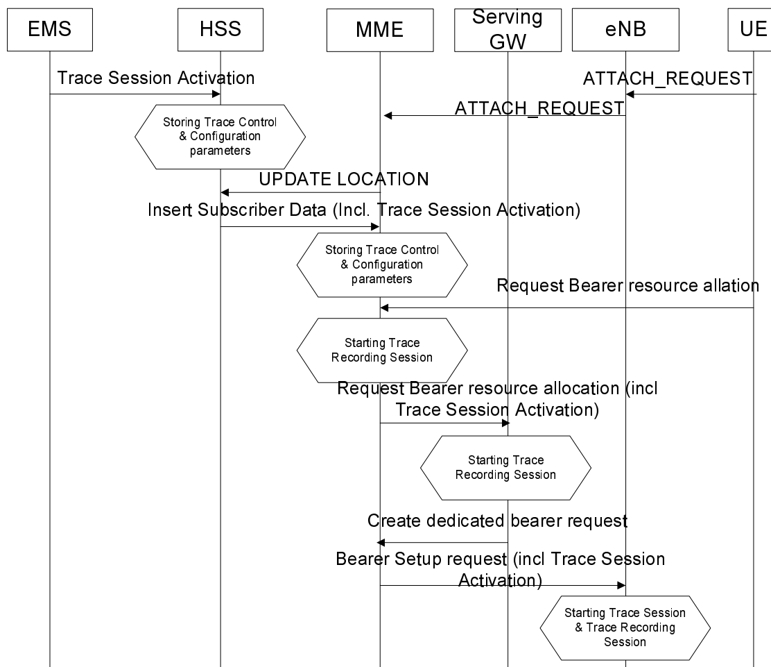
Figure 4.1.2.10.1: Trace Session activation procedure in EPC:
