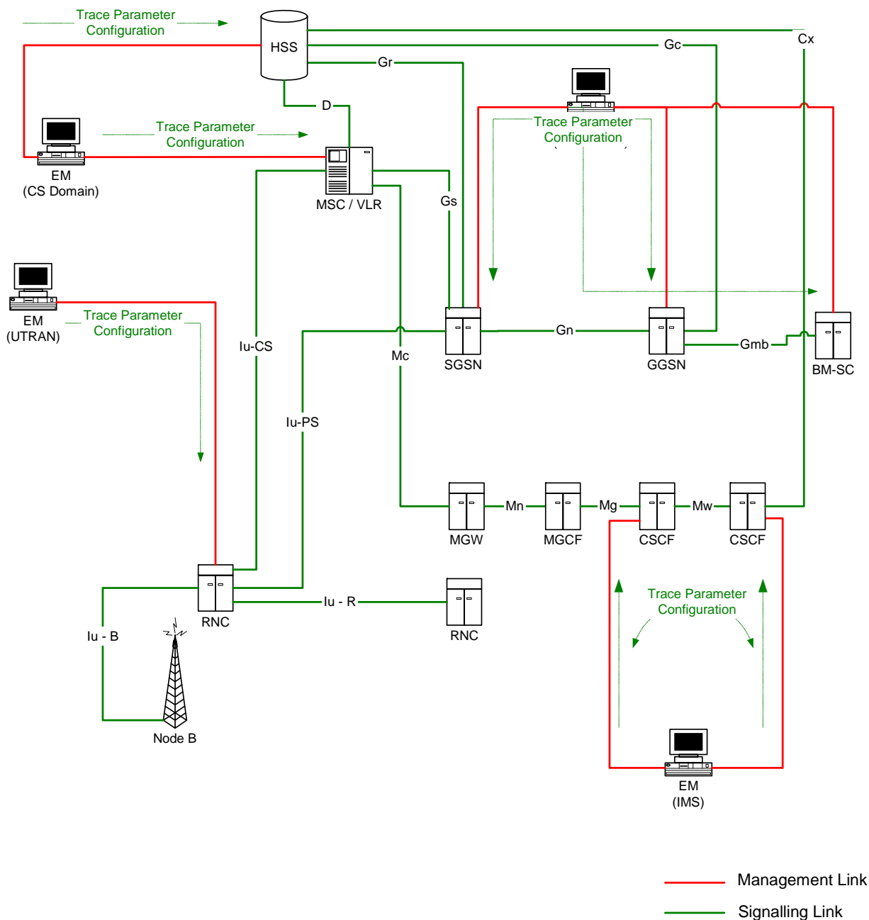
Figure 4.1.1.1: Overview of management activation for an UMTS system
