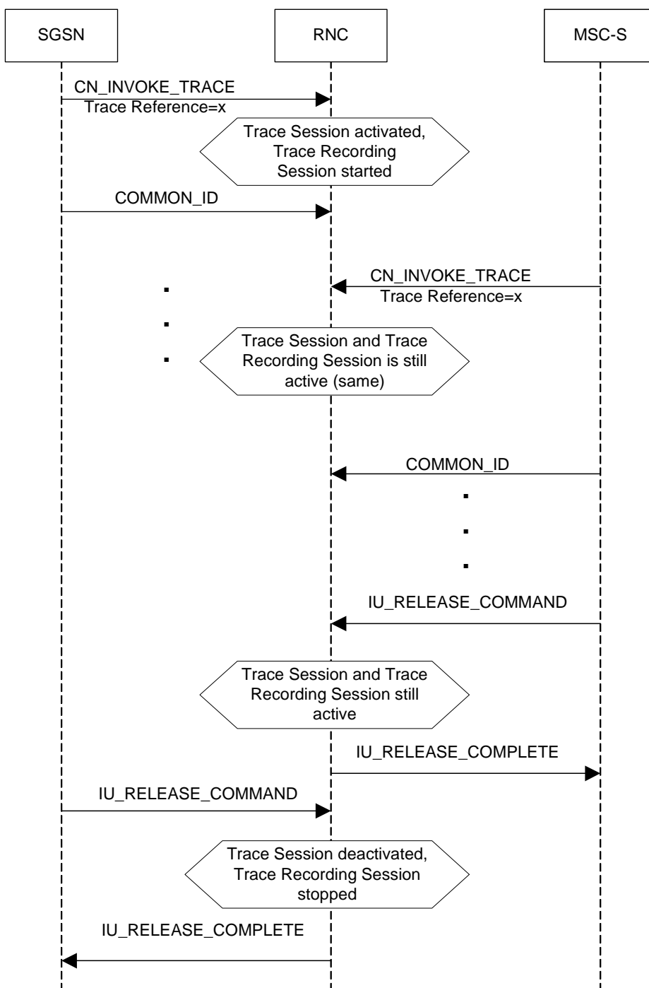
Figure 4.1.4.2.2: Trace session deactivation (Signalling) in UTRAN 2
