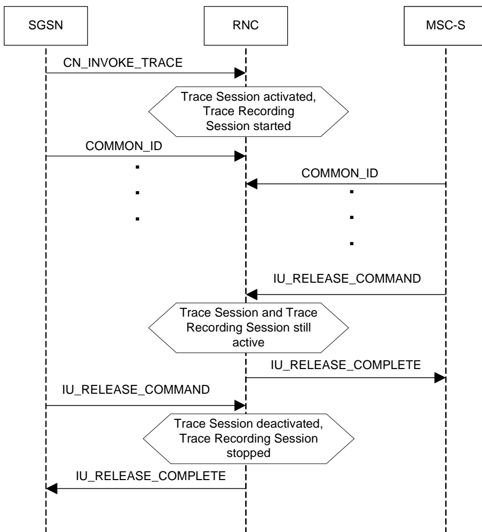
Figure 4.1.4.2.1: Trace session deactivation (Signalling) in UTRAN 1
