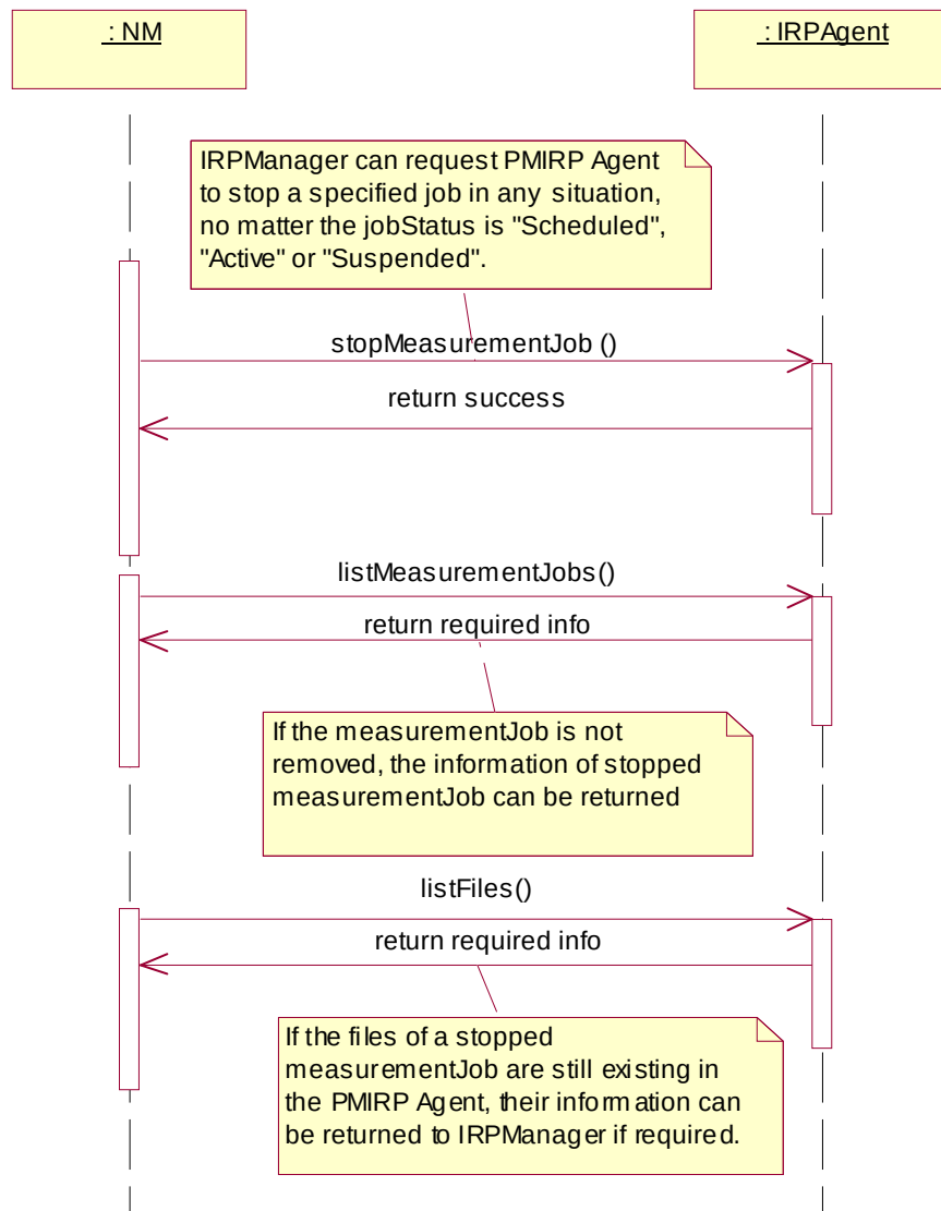
Figure 8.3: Scenario3 of Performance Management
