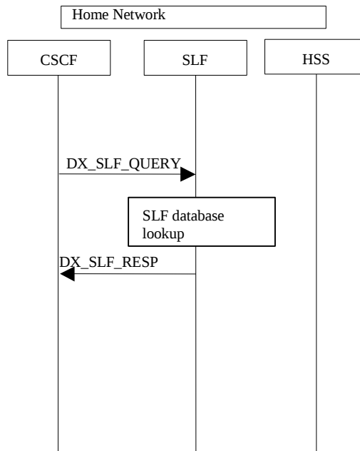
Figure 18: Routing information interrogation procedure from CSCF
