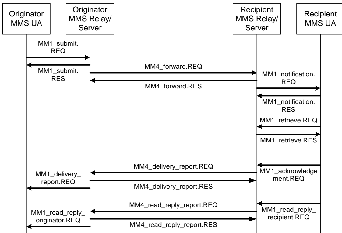
Figure 4.2: Example Abstract Message Flow
