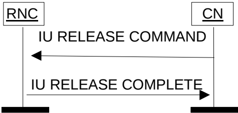
Figure: Iu Release procedure. Successful operation.
