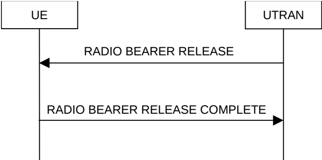
Figure: Radio Bearer Release, normal case
