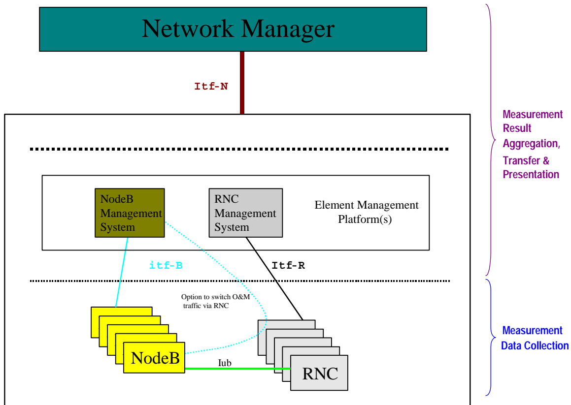
Figure 1: UTRAN Performance management concept
