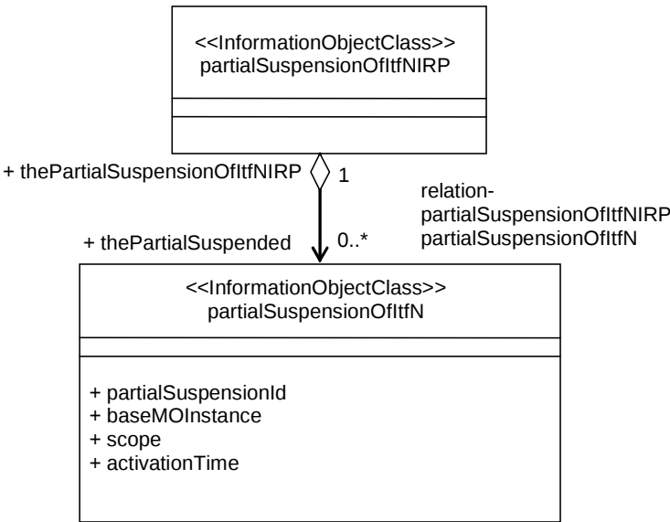
Figure 5.2.1-1: Class Diagram
