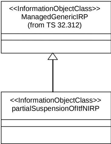
Figure 5.2.2-1: Inheritance Diagram
