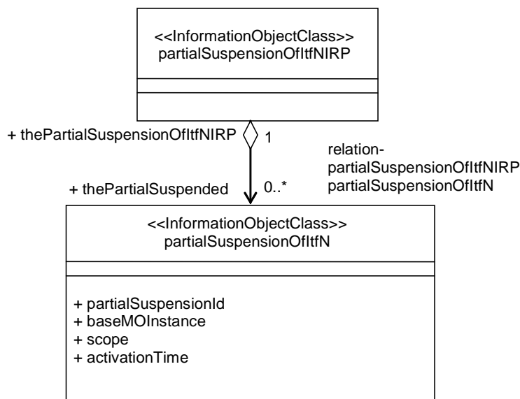
Figure 5.2.1-1: Class Diagram
