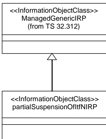
Figure 5.2.2-1: Inheritance Diagram
