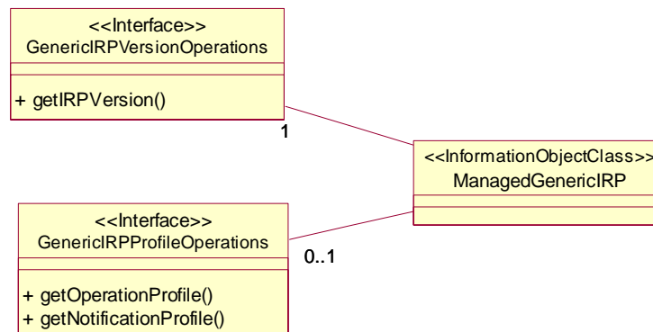
Figure 5: Class diagram representing interfaces
