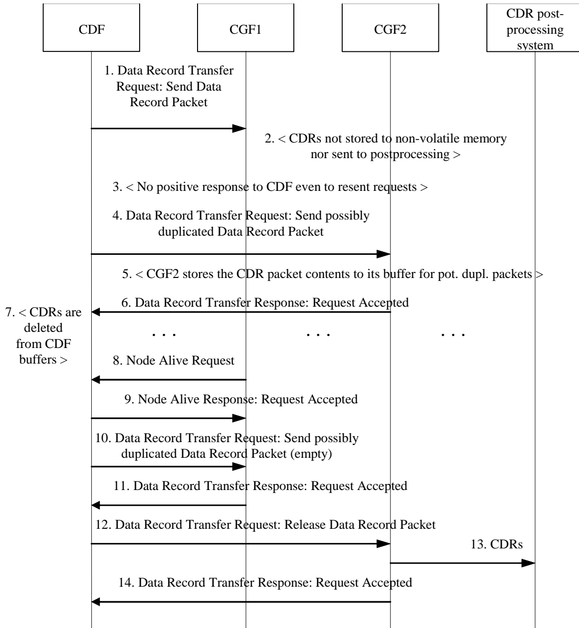
Figure 5.2.2.1: Duplicate prevention case: CDR sending via CGF1 had not succeeded
