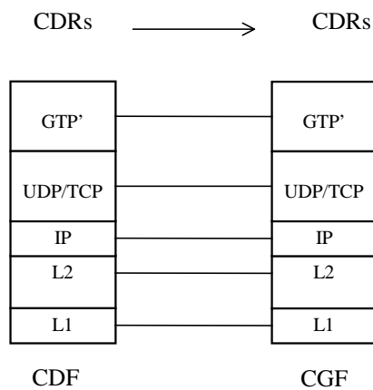
Figure 5.1.2.1.1: Protocol layers between the CDF and the CGF
