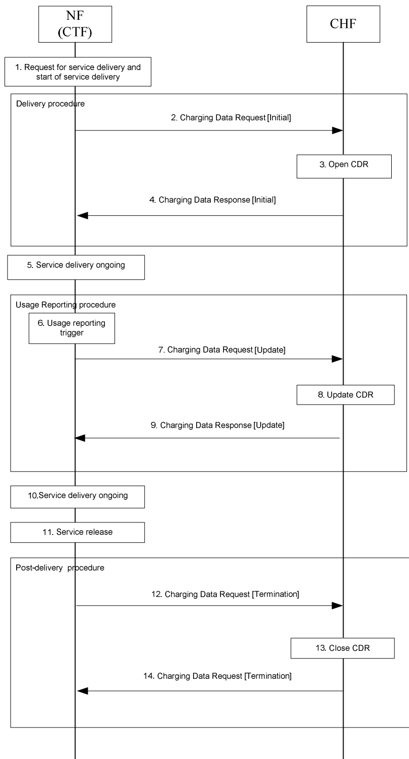
Figure 5.1.2.2.1: Offline charging
