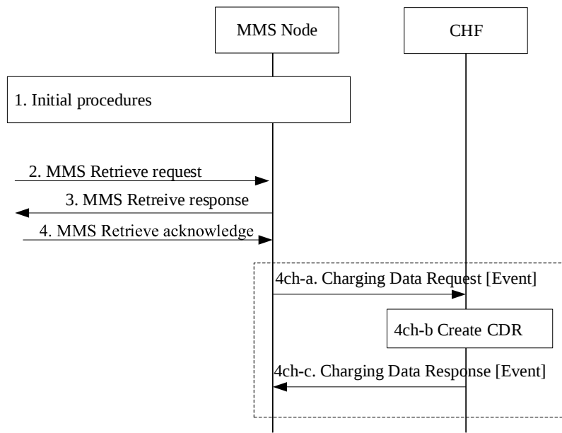
Figure 5.4.2.3.3 MMS retrieval from MMS Node for PEC
