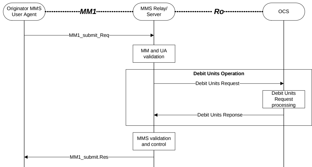
Figure 5.3.2.1.1: MMS online charging scenario for MM submission
