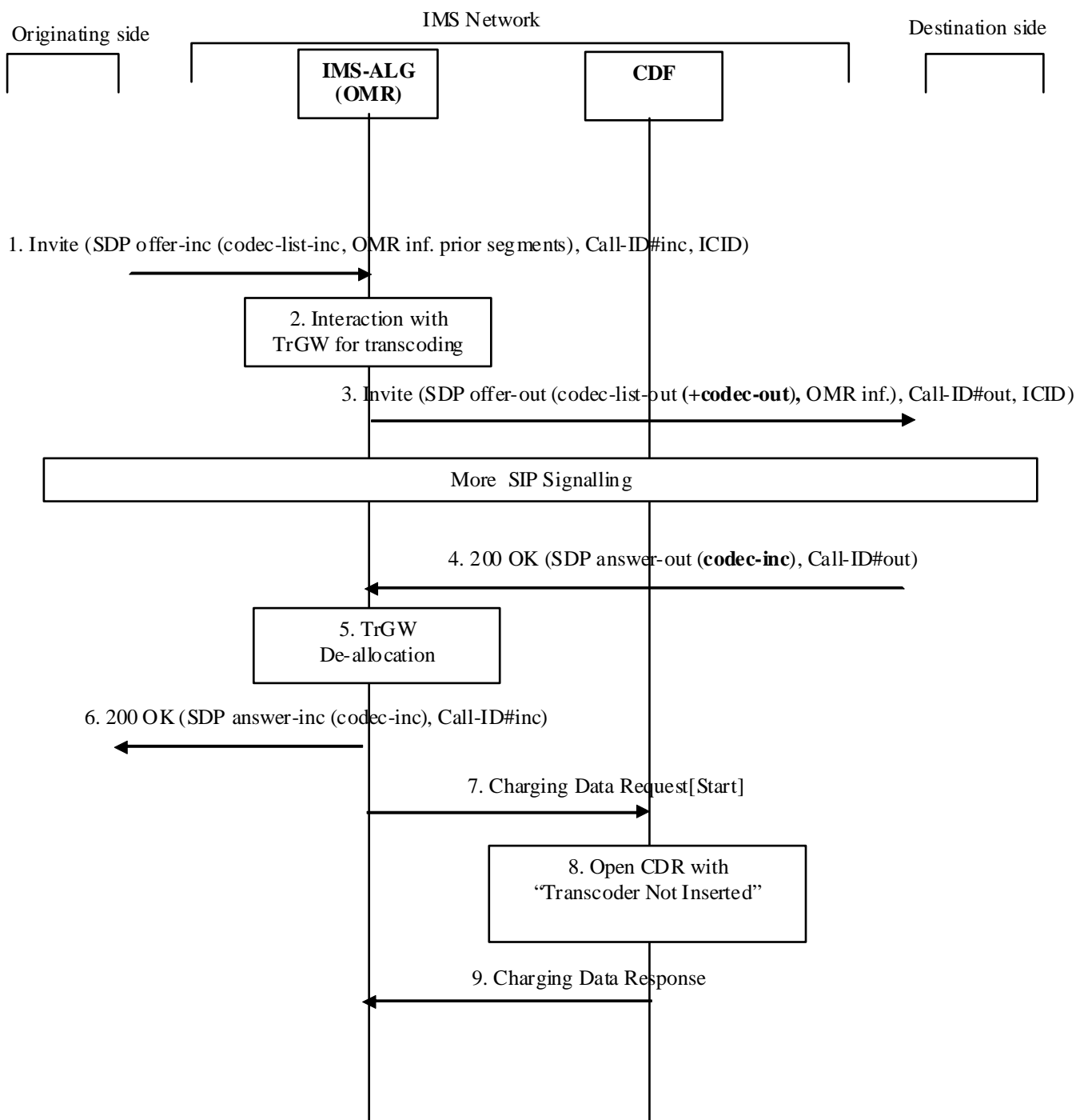
Figure 5.2.2.19.4.2.1: Message sequence chart for session establishment with transcoder offered by IMS-ALG is not selected
