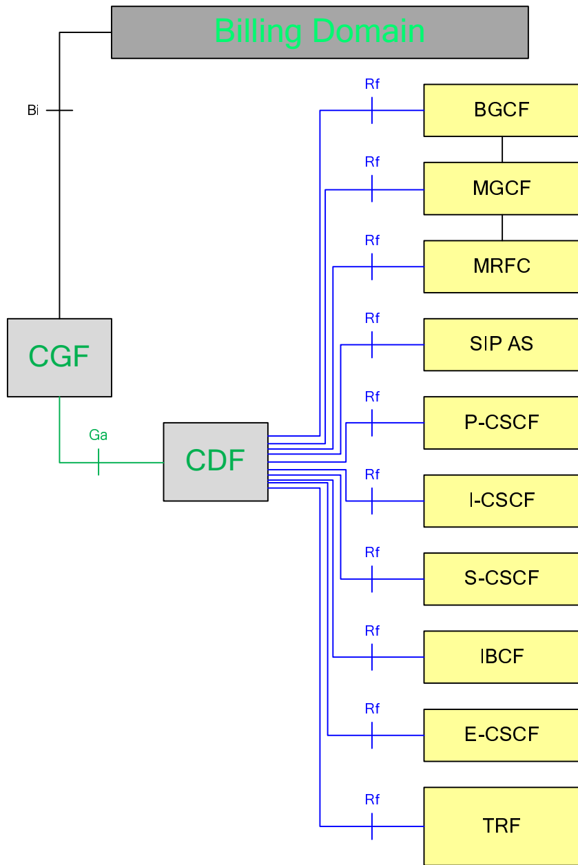
Figure 4.2: IMS offline charging architecture
