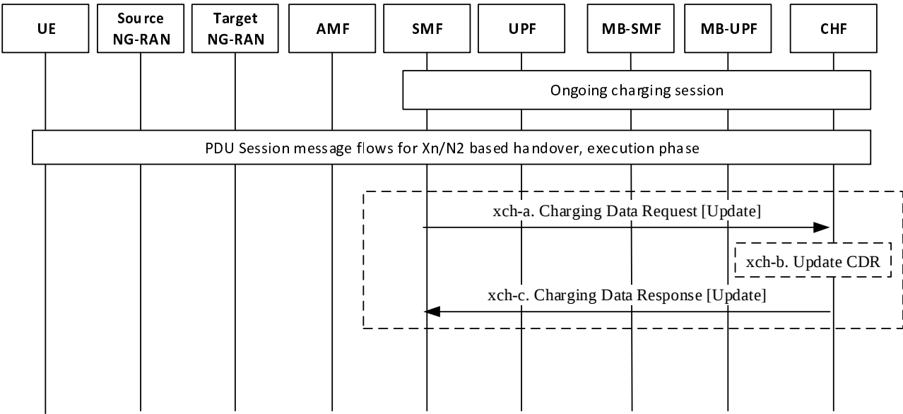
Figure 5.2.2.24.3.1: Xn/N2 based handover, execution phase
