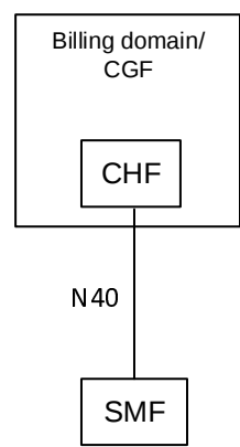
Figure 4.2.2: 5G data connectivity converged charging architecture non-roaming reference point representation
