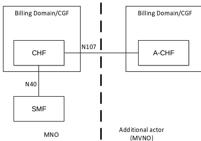
Figure 4.2.6c: 5G data connectivity converged charging architecture in additional actor (i.e. MVNO owning a CHF, referred to as A-CHF) scenario in reference point representation
