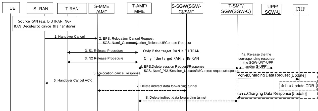
Figure 5.2.2.11.4.1: Handover Cancel
