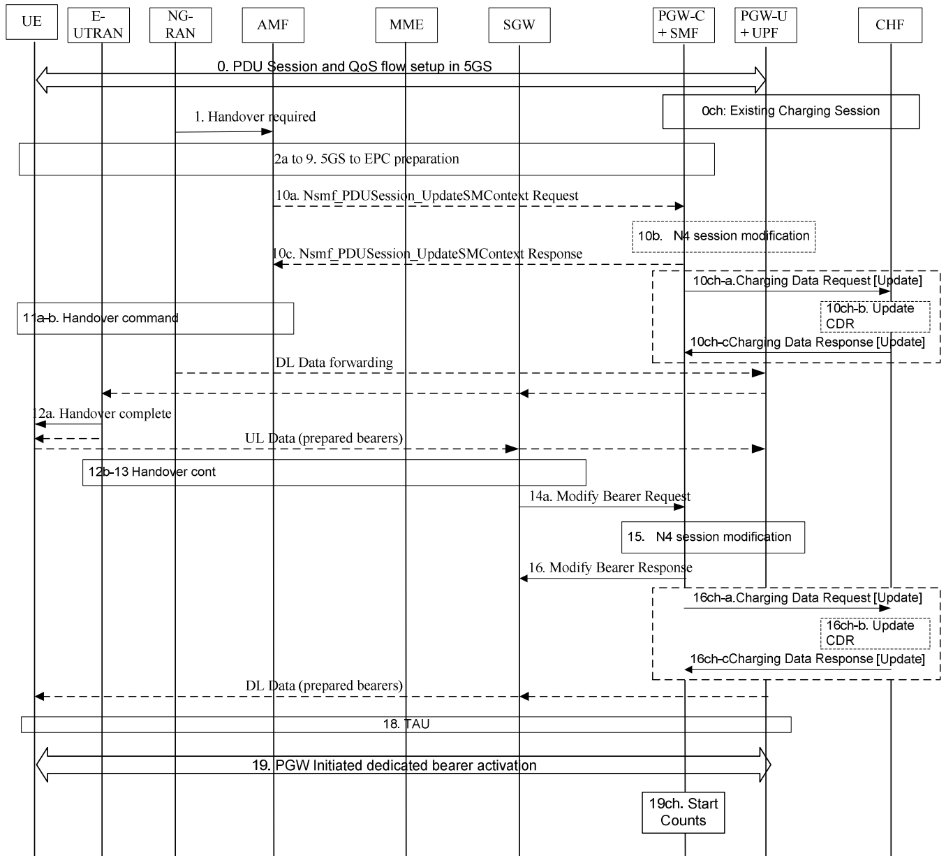
Figure 5.2.2.11.2.1: 5GS to EPS handover using N26
