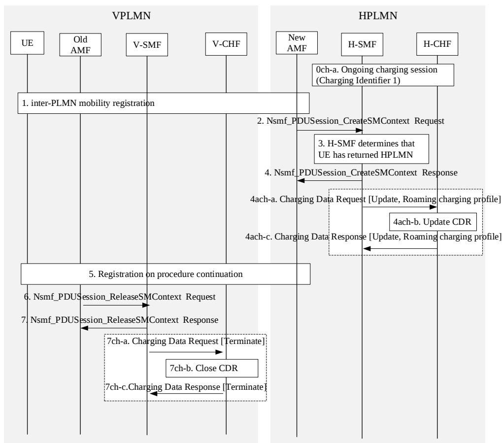
Figure 5.2.2.12.9.1: Roaming Home routed PDU session inter-PLMN V-SMF removal
