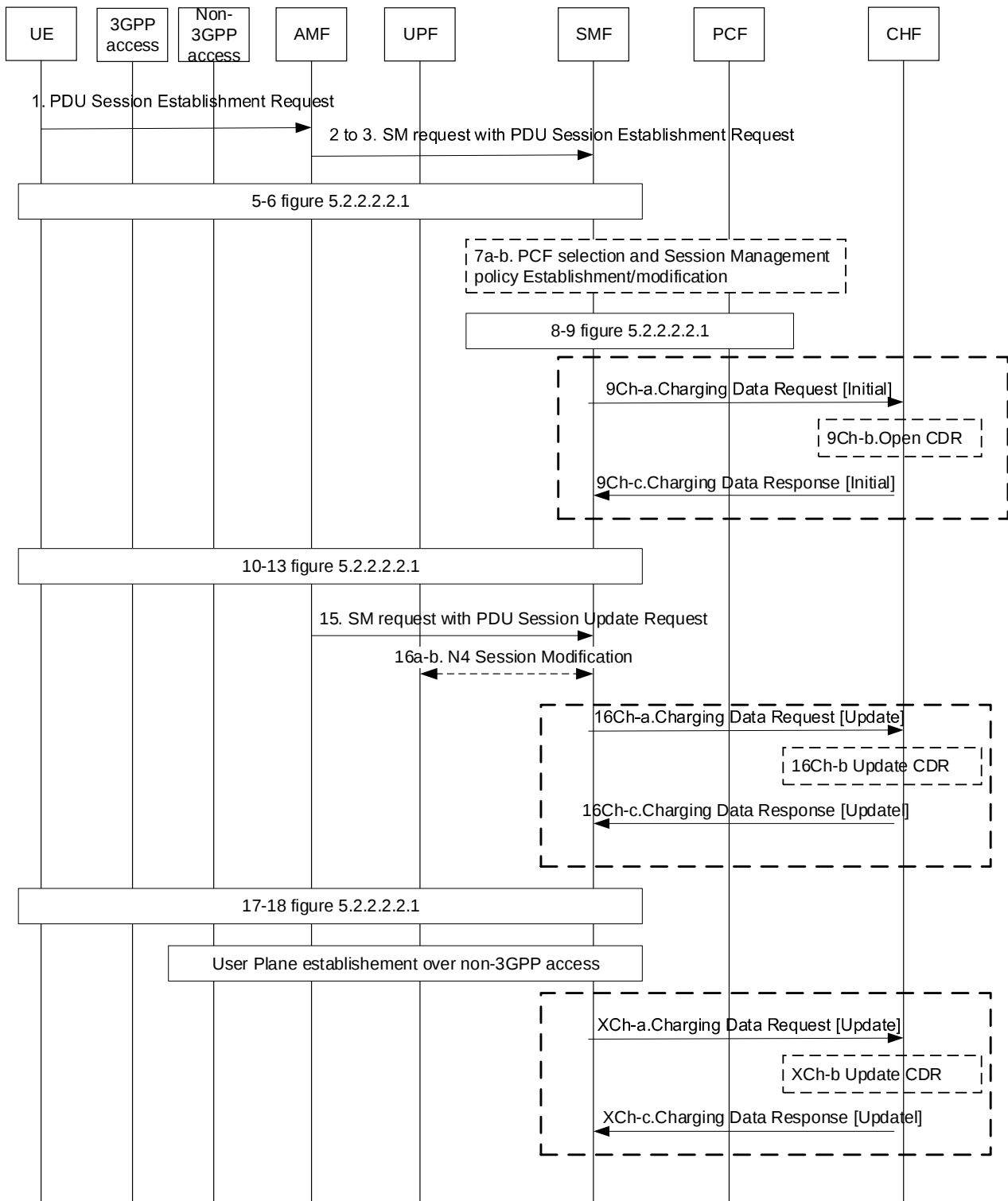
Figure 5.2.2.15.2.1: UE Requested MA PDU session establishment
