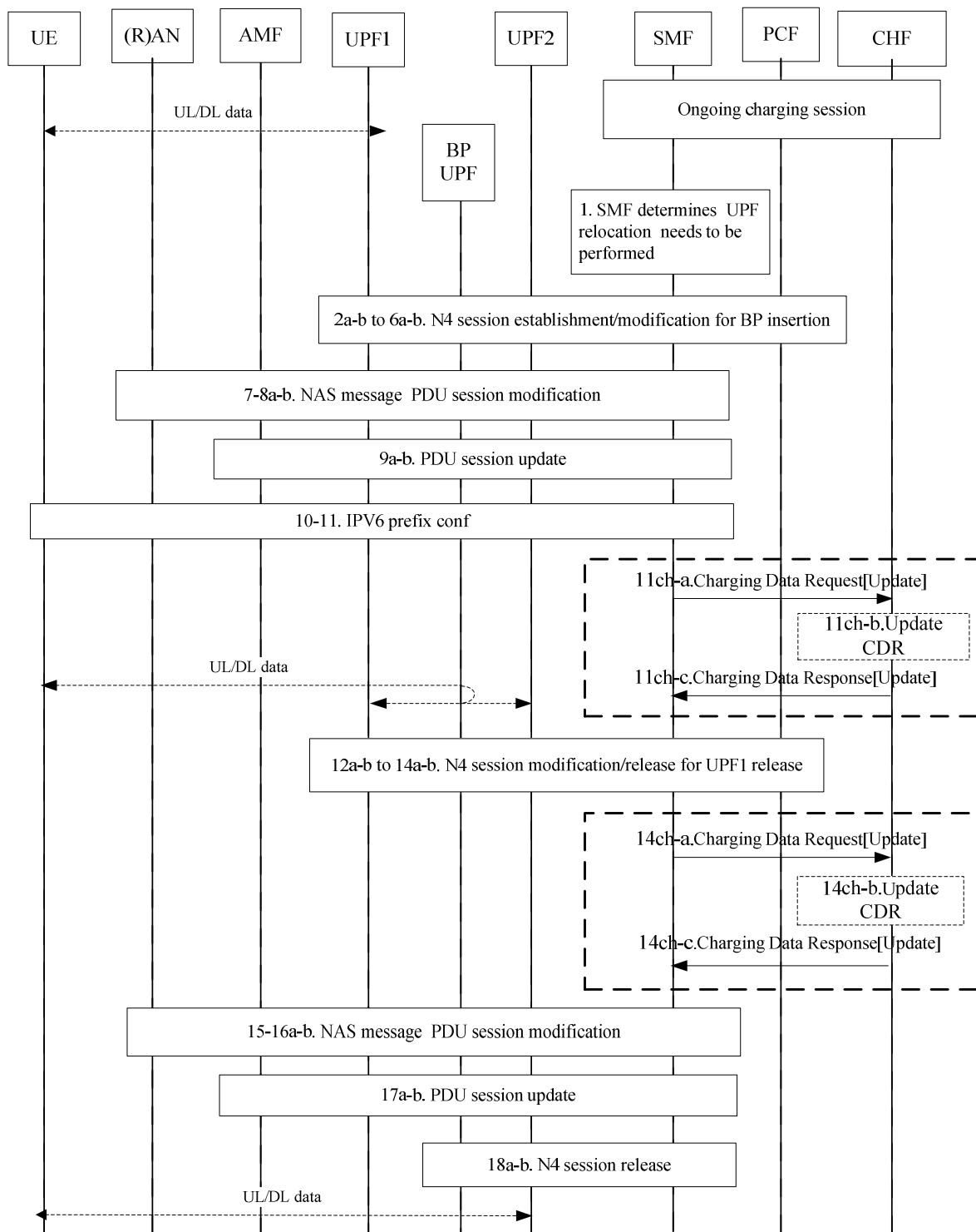
Figure 5.2.6.2.1: PDU session anchor relocation in SSC mode 3 with IPv6 Multi homed PDU Session
