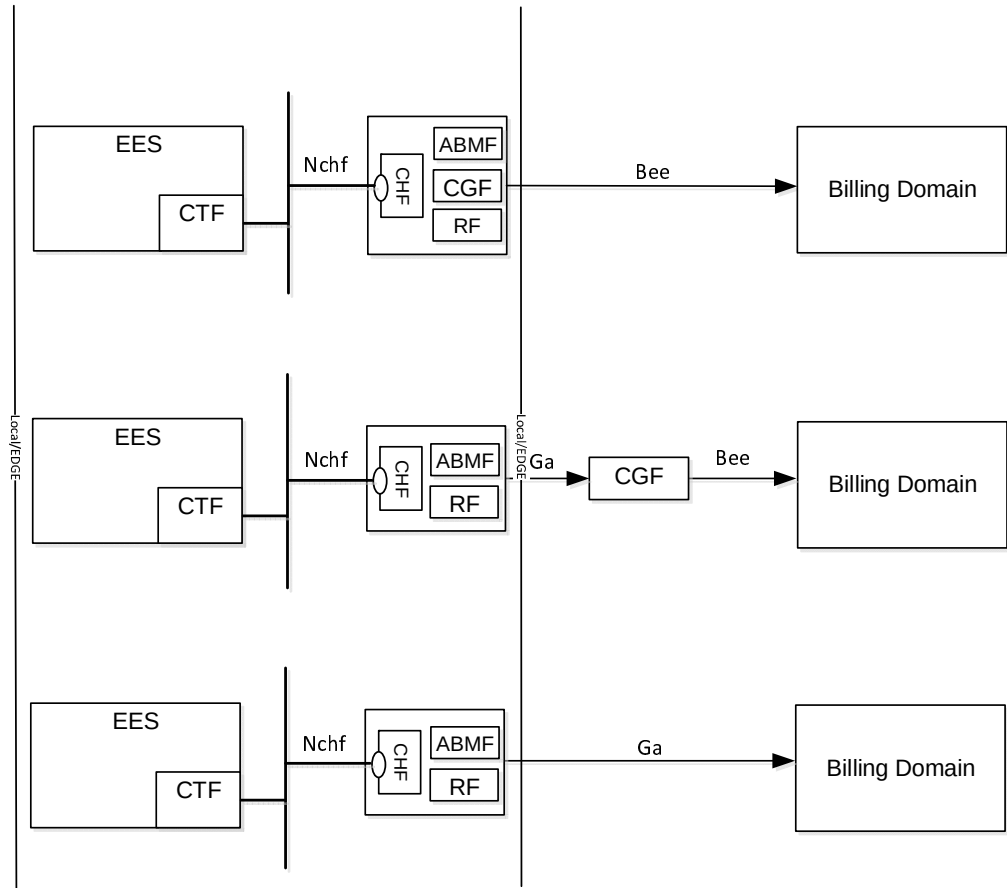
Figure F.2.2-1: Converged charging architecture --- distributed deployment example scenario
