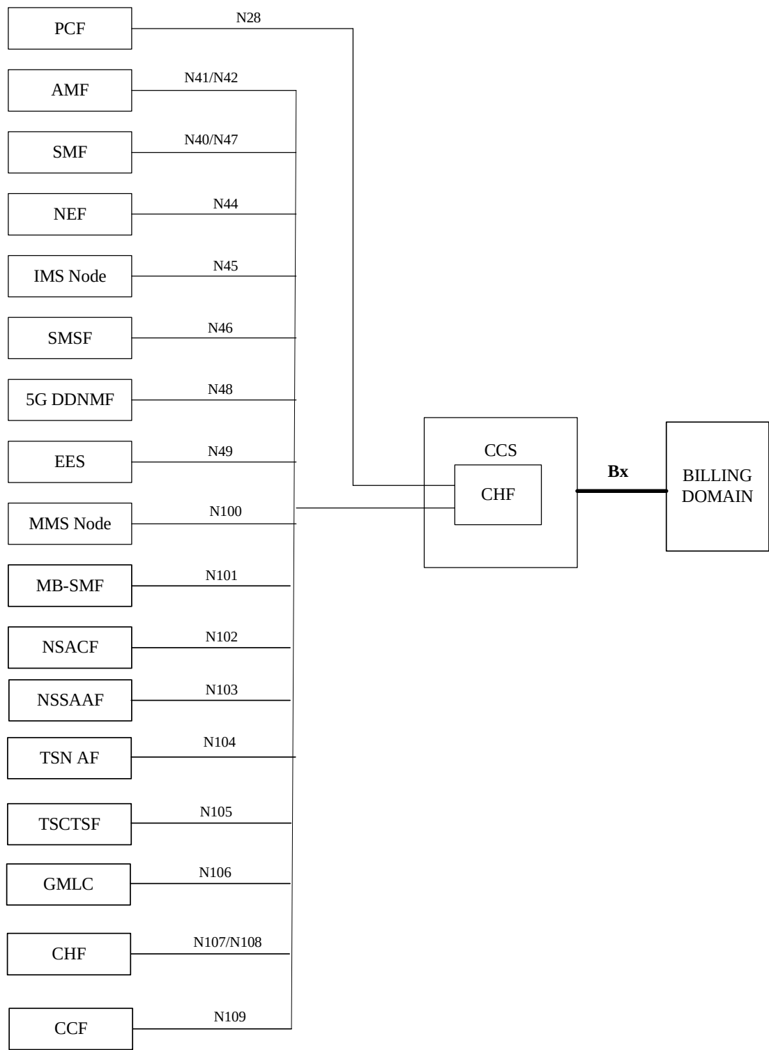
Figure 4.2.3.2: Logical ubiquitous charging architecture and information flows for 5G systems – reference point representation
