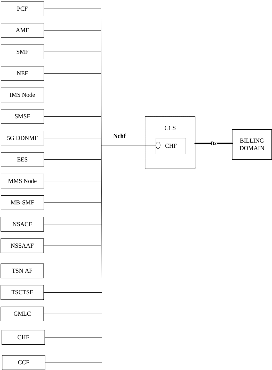
Figure 4.2.3.1: Logical ubiquitous charging architecture and information flows for 5G systems – service based representation
