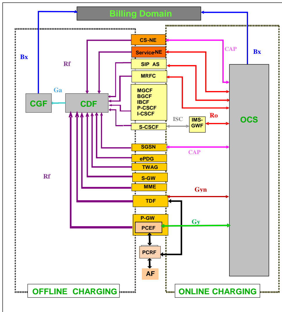
Figure 4.2.1: Logical ubiquitous charging architecture and information flows
