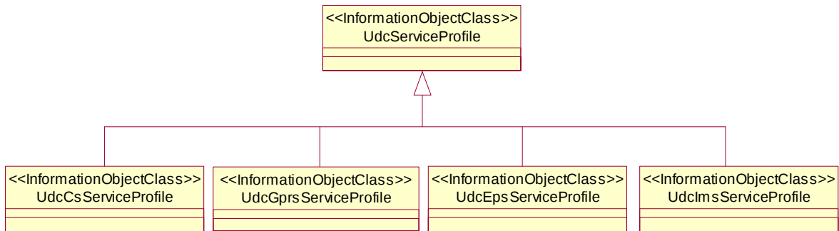
Figure 5.2.2-1: UdcServiceProfile inheritance
