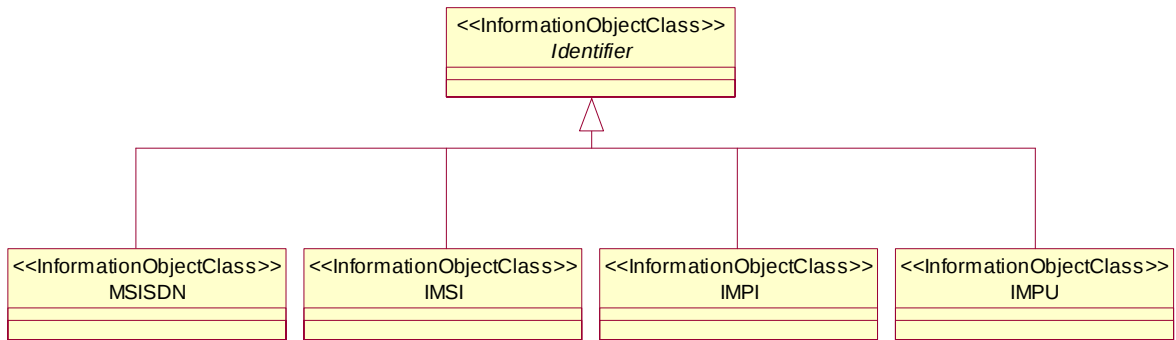
Figure 5.2.2-2: Identifier inheritance
