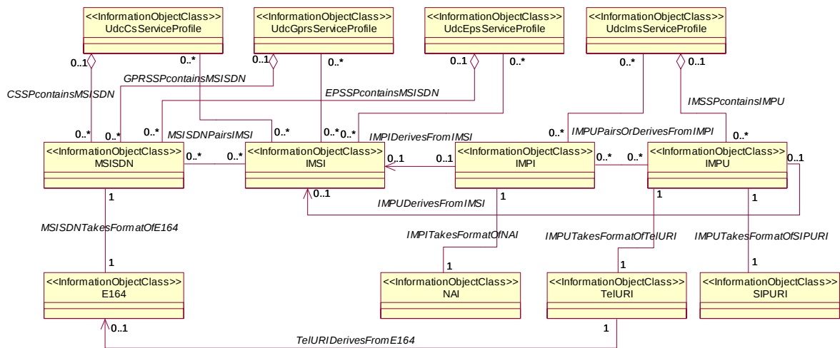
Figure 5.2.1-2: Identifiers
