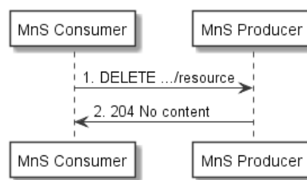
Figure 5.4-1: Flow for deleting a resource
