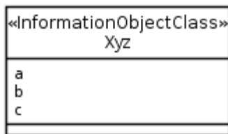
Figure 5.2.1.2-1: Attribute notation
