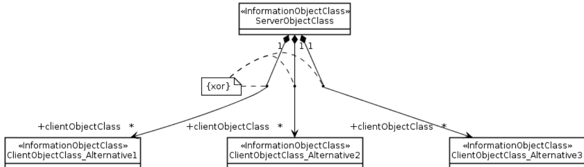
Figure 5.2.10.2-1: {xor} notation
