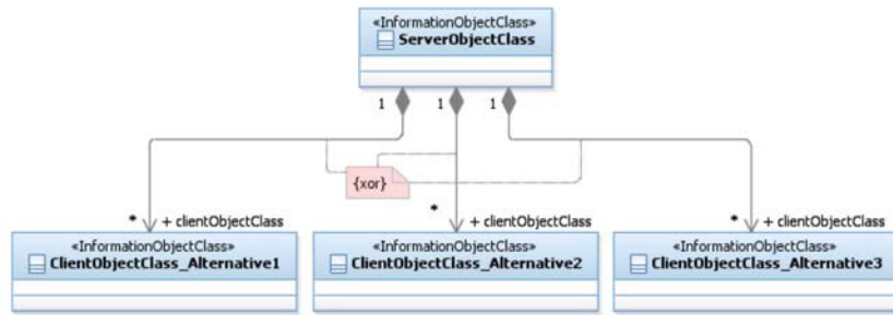
Figure 5.2.10.2-1: {xor} notation
