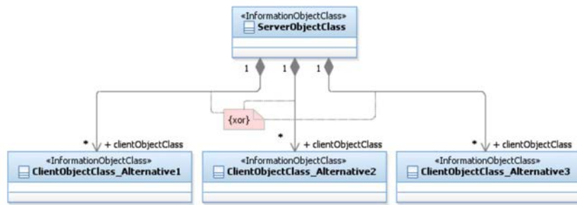
Figure 5.2.10.2-1: {xor} notation
