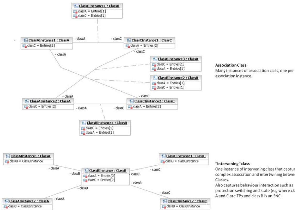
Figure C.1.1-2: Instance view of "intervening class"
