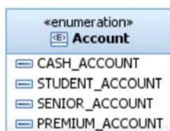
Figure 5.3.5.2-1: <<enumeration>> notation
