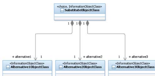
Figure 5.3.6.2-1: Information model element example using <<choice>> notation
