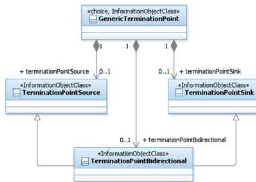
Figure 5.3.6.2-3: Sink/source/bidirectional termination points example using «choice» notation
