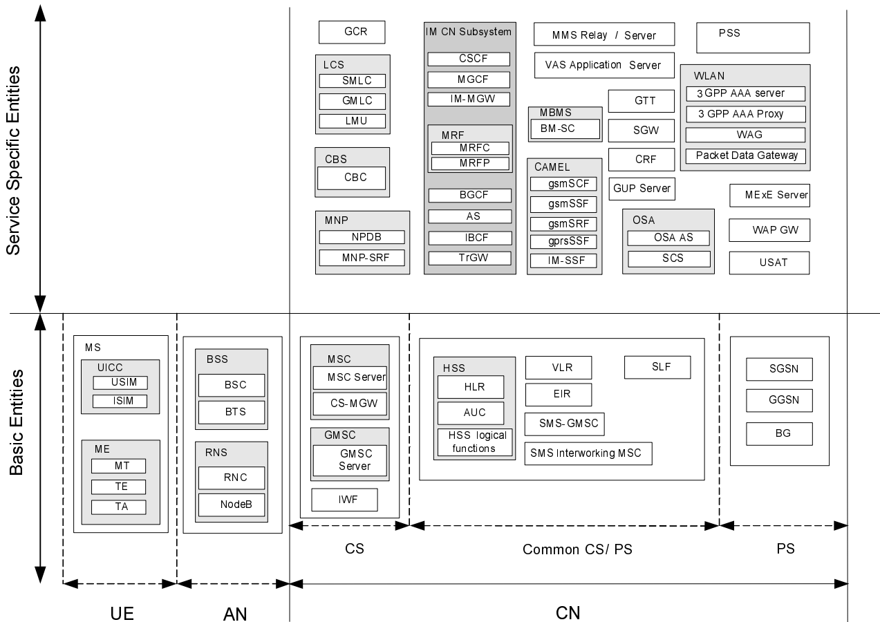
Figure 7.3.3.1: Examples of entities of the mobile system to be managed
