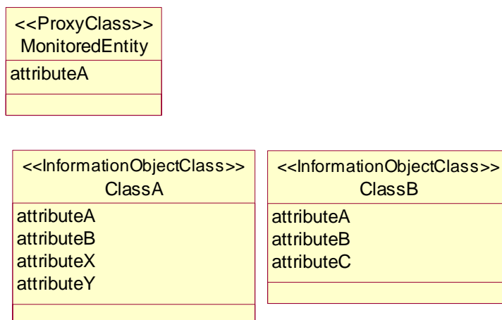
Figure : <<ProxyClass>>
