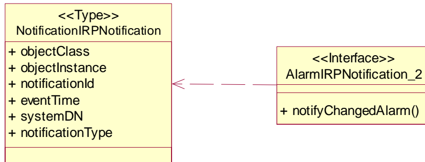
Figure 2: <<Type>> Notation
