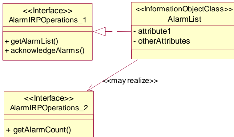
Figure : Relationship realize and <<may realize>> Notations
