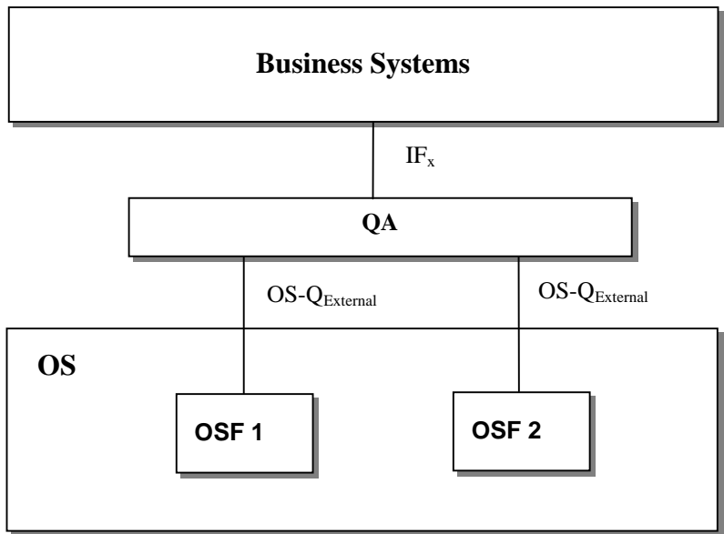
Figure 8.5: Business Systems interconnection architecture
