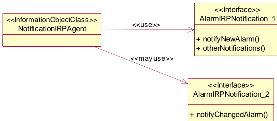
Figure : <<use>> and <<may use>> Notation
