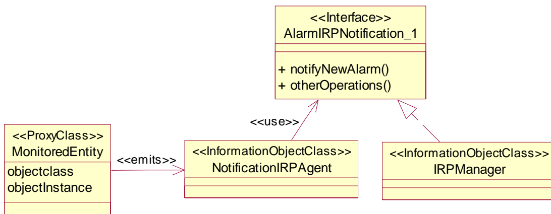
Figure : <<use>>, <<emits>> and realize relationship Notation
