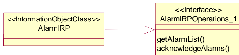
Figure : <<Interface>> Notation
