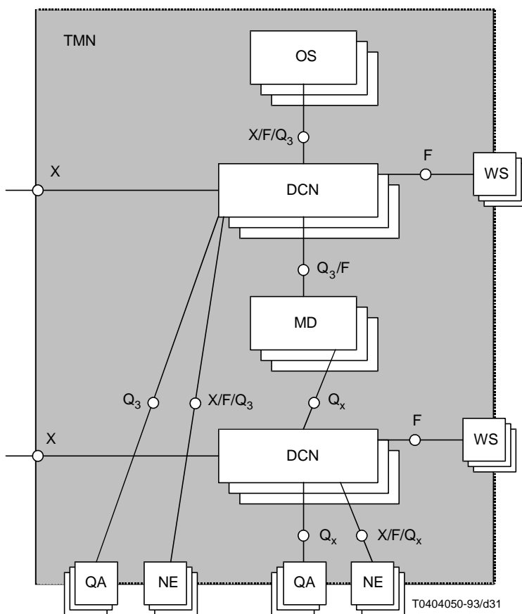
Figure A.1: Examples of interfaces for the TMN physical architecture M.3010 [1]
