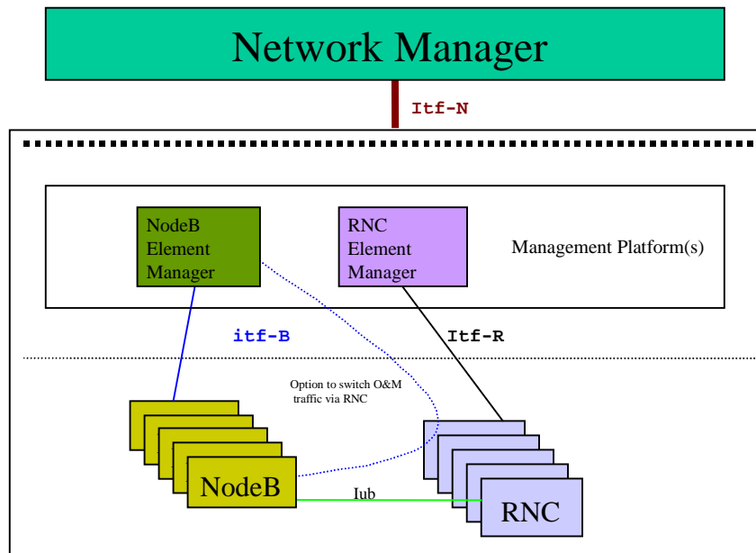
Figure 2: Radio Network Management Interfaces
