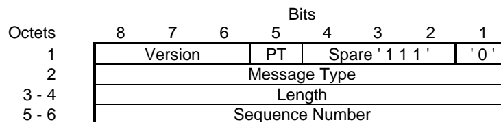
Figure 12: GTP' header
