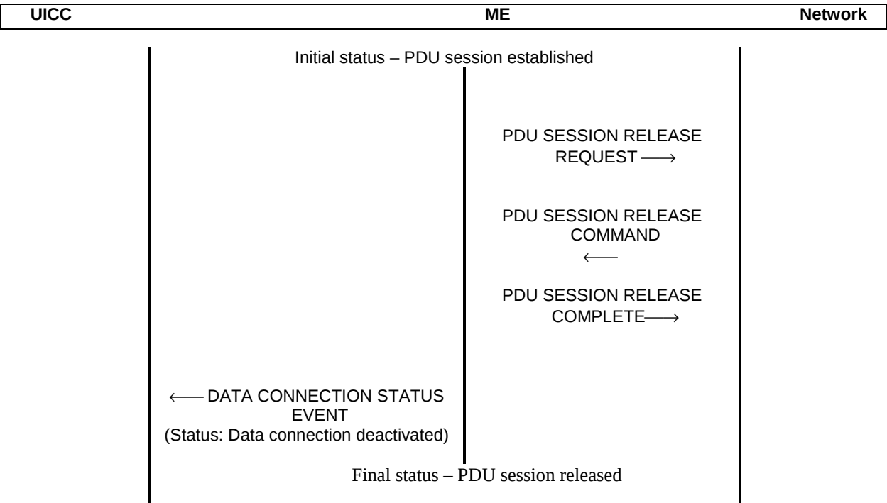
Figure T.4.3 MS Initiated PDU session release procedure
