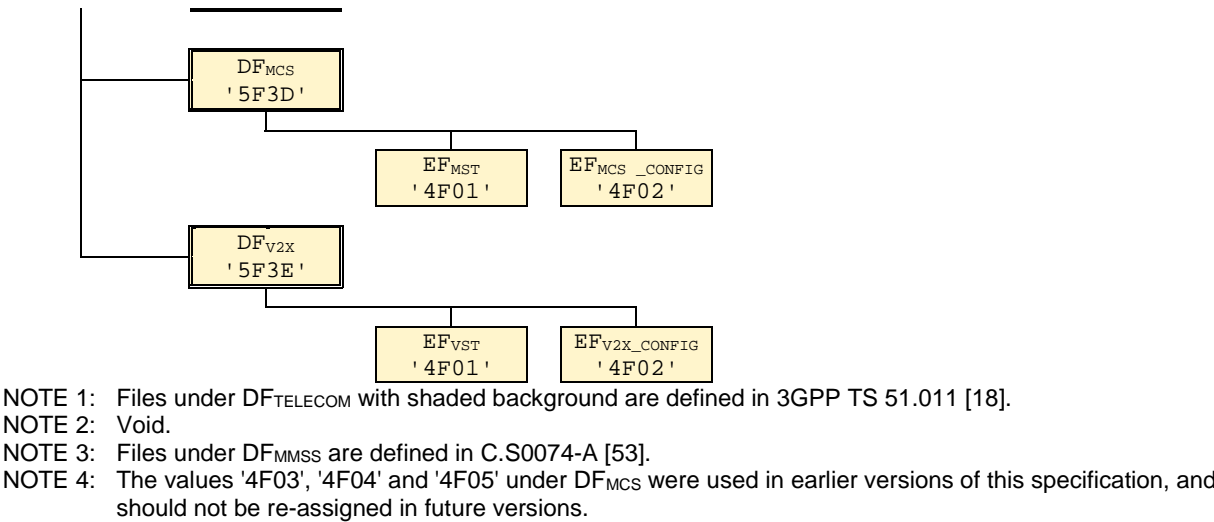
Figure 4.1: File identifiers and directory structures of UICC
