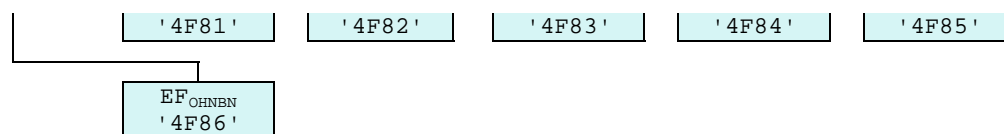
Figure 4.2: File identifiers and directory structures of USIM
