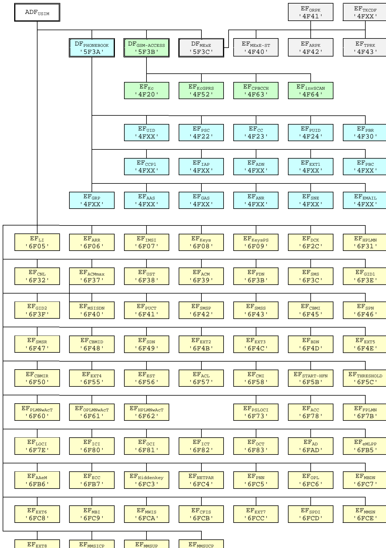
Figure 4.1: File identifiers and directory structures of UICC
