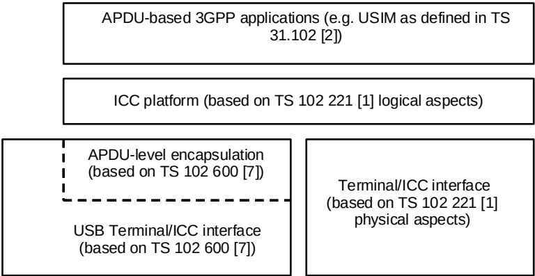
Figure 1: Terminal/UICC interface
