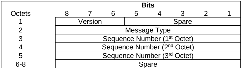
Figure 7.1.2.2-1: Message Header
