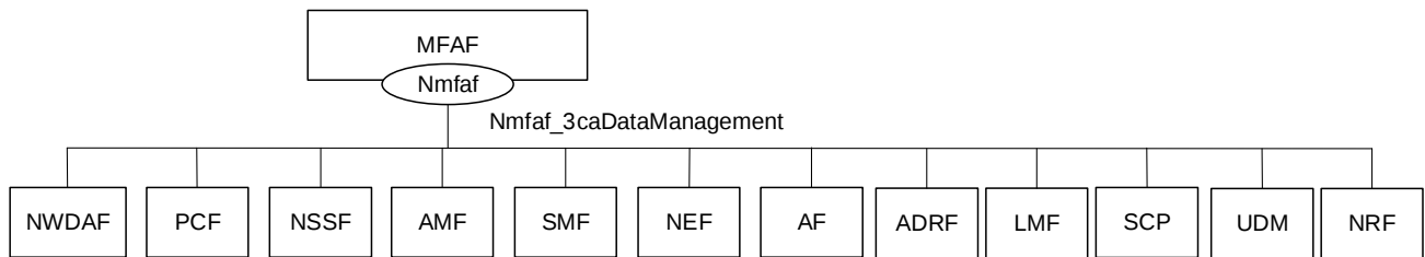
Figure 4.3.1.2-1: Reference Architecture for the Nmfa3caDataManagement Service; SBI representation
