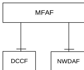
Figure 4.2.1.2-2: Reference Architecture for the Nmfaf_3daDataManagement Service; reference point representation
