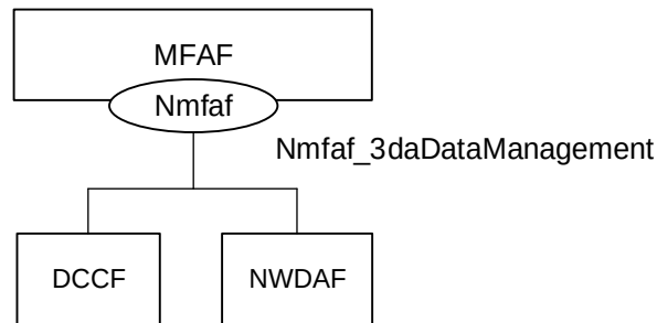
Figure 4.2.1.2-1: Reference Architecture for the Nmfa3daDataManagement Service; SBI representation
