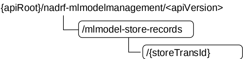
Figure 5.2.3.1-1: Resource URI structure of the Nadr_f_MLModelManagement API
