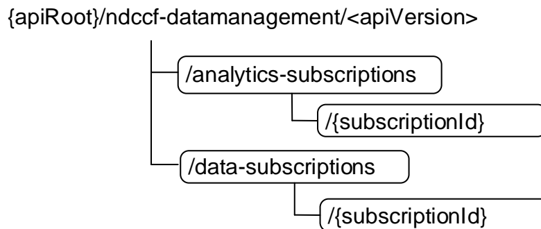
Figure 5.1.3.1-1: Resource URI structure of the Ndcf_DataManagement API
