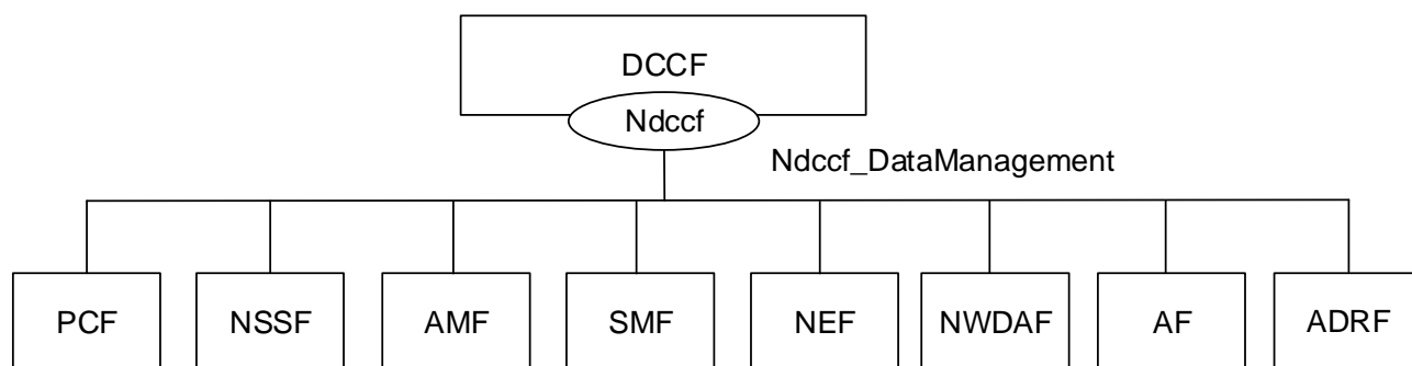
Figure 4.2.1.2-1: Ndccf_DataManagement service architecture, SBI representation
