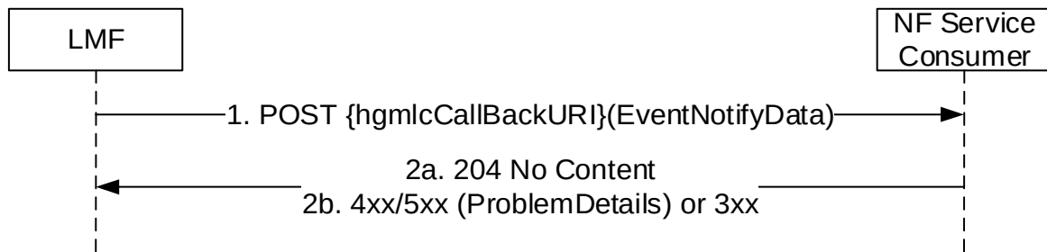
Figure 5.2.2.3.2-1: EventNotify Request
