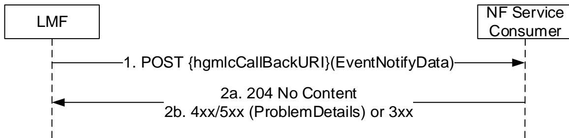
Figure 5.2.2.3.2-1: EventNotify Request
