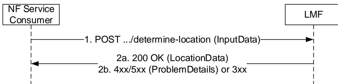
Figure 5.2.2.2.2-1: DetermineLocation Request
