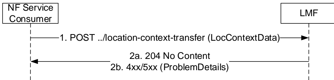
Figure 5.2.2.5.2-1: LocationContextTransfer Request
