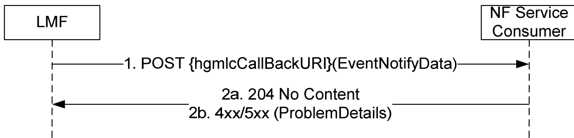
Figure 5.2.2.3.2-1: EventNotify Request
