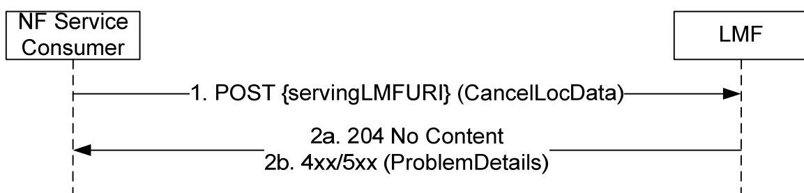
Figure 5.2.2.4.2-1: CancelLocation Request
