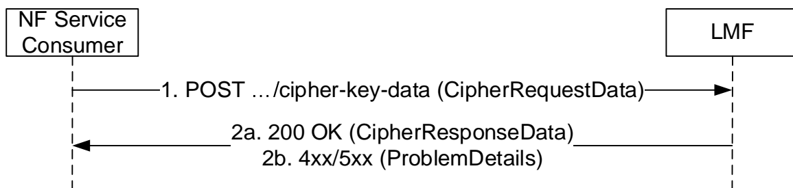
Figure 5.3.2.2.2-1: CipherringKeyData Request
