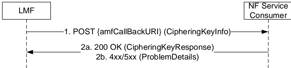
Figure 5.3.2.2.3-1: CipherringKeyData Notify
