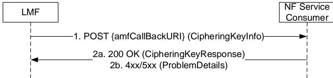
Figure 5.3.2.2.3-1: CipherringKeyData Notify
