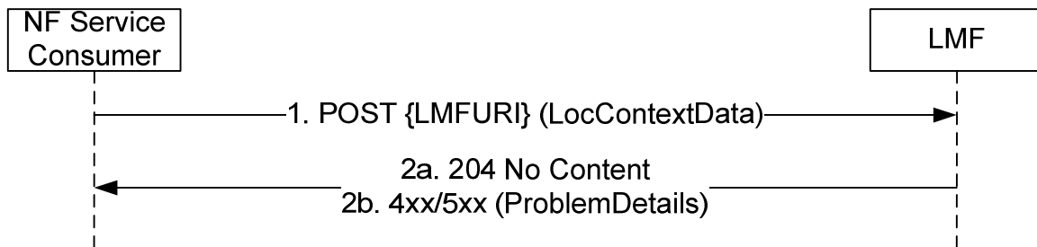
Figure 5.2.2.5.2-1: LocationContextTransfer Request
