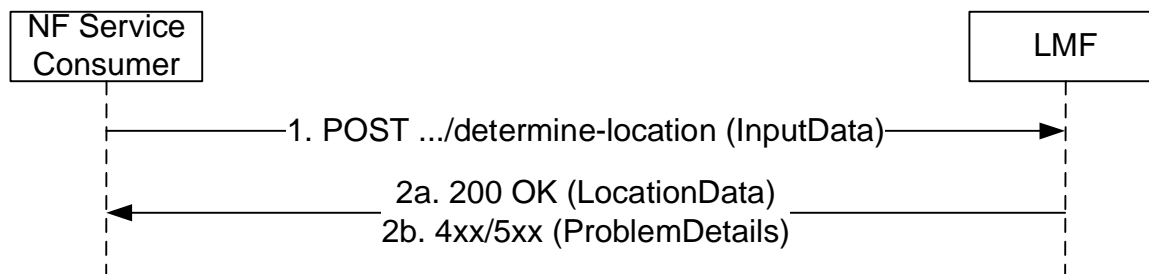
Figure 5.2.2.2.2-1: DetermineLocation Request
