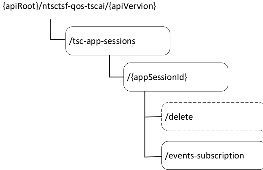
Figure 6.2.3.1-1: Resource URI structure of the Ntsctsf_QoSandTSCAssistance API
