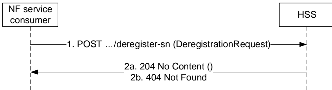
Figure 5.4.2.2-1: SN Deregistration
