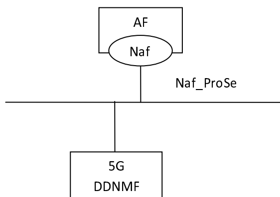
Figure 4-1: Naf_ProSe Service architecture, SBI representation
